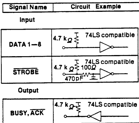
Figure N-2. Sample circuit for parallel interface.
